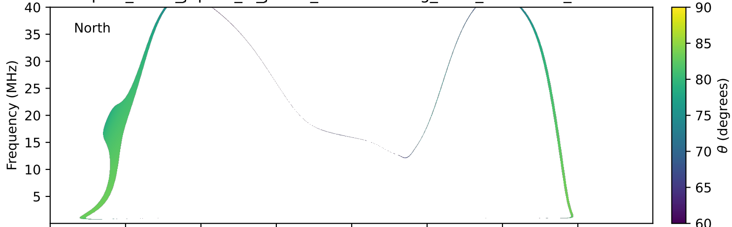
expres_earth_jupiter_io_jrm09_lossc-wid1deg_3kev_19920930_v11.cdf
