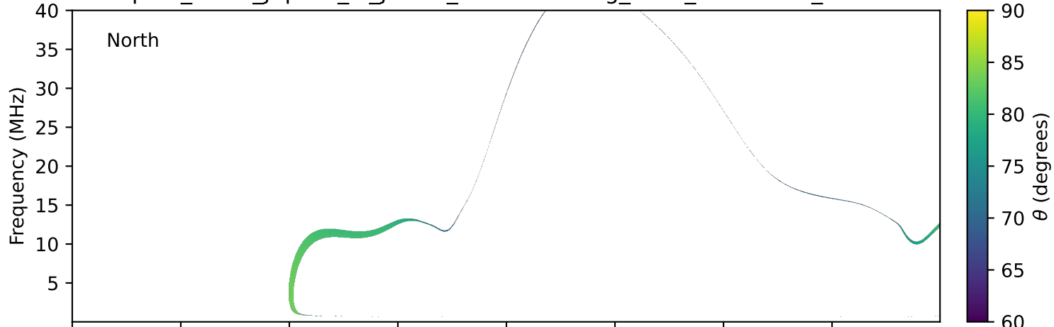
expres_earth_jupiter_io_jrm09_lossc-wid1deg_3kev_19920928_v11.cdf
