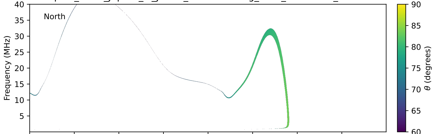
expres_earth_jupiter_io_jrm09_lossc-wid1deg_3kev_19920916_v11.cdf
