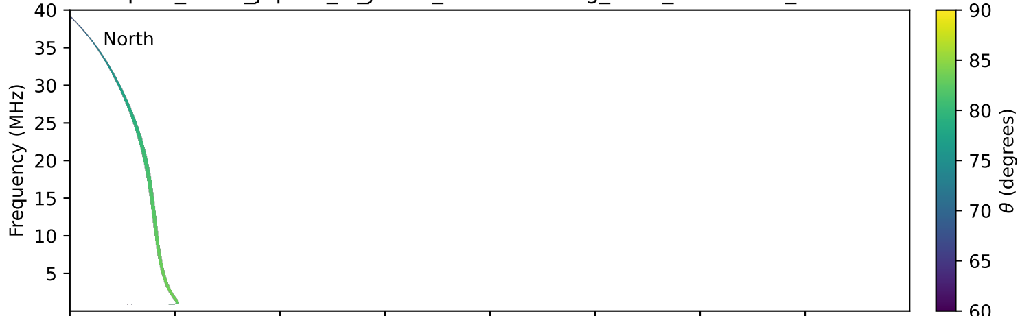
expres_earth_jupiter_io_jrm09_lossc-wid1deg_3kev_19920913_v11.cdf
