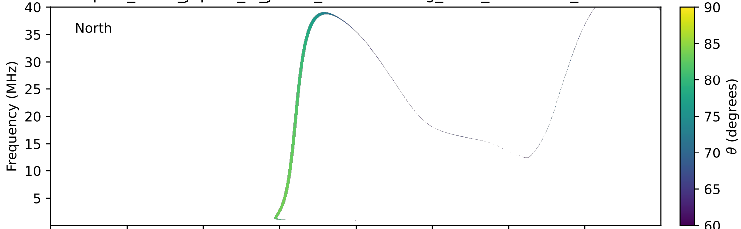
expres_earth_jupiter_io_jrm09_lossc-wid1deg_3kev_19920912_v11.cdf
