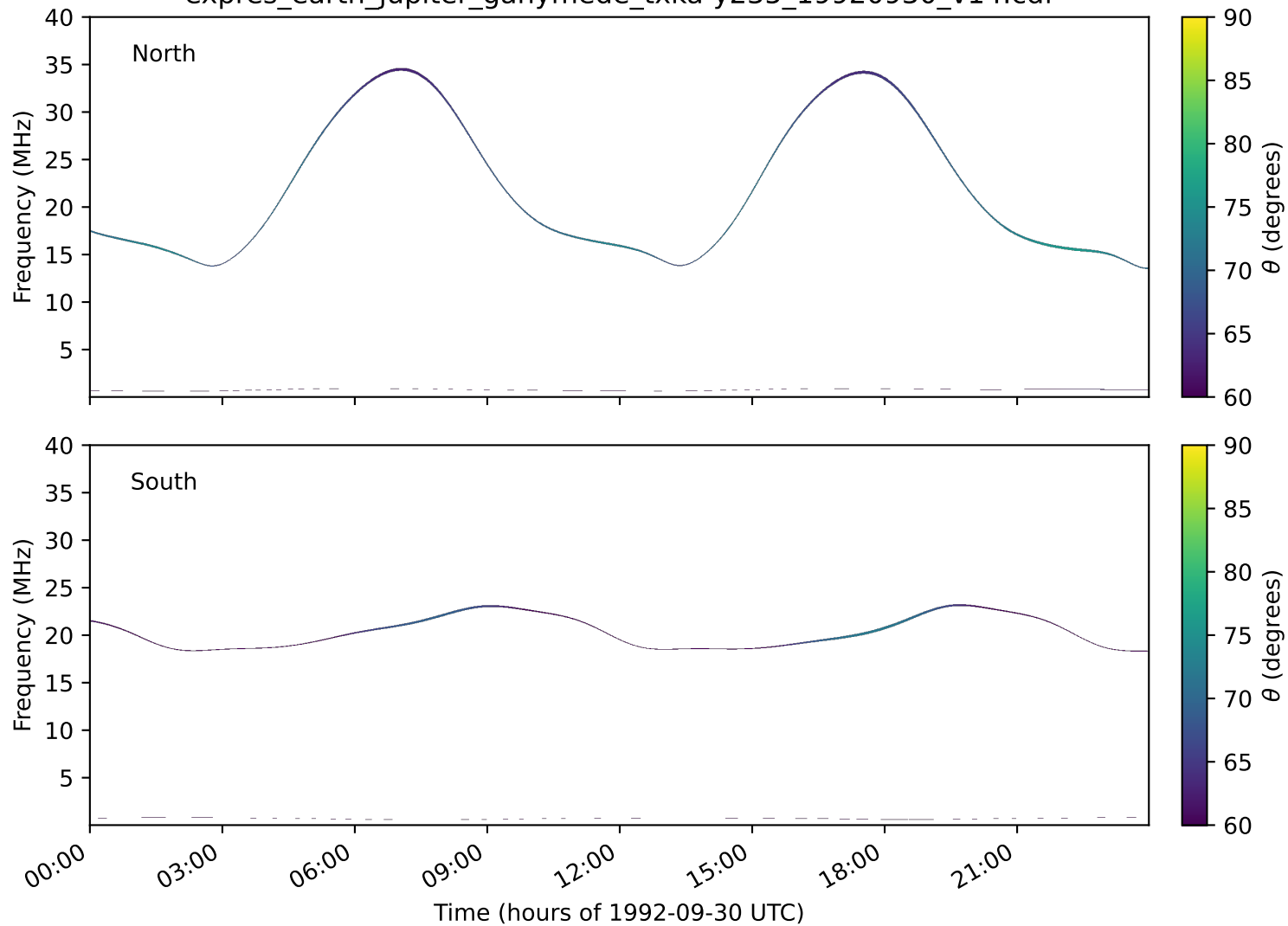
expres_earth_jupiter_ganymede_txka-y235_19920930_v14.cdf
