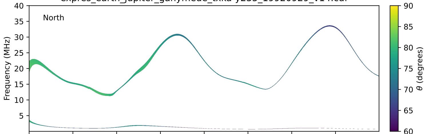
expres_earth_jupiter_ganymede_txka-y235_19920929_v14.cdf
