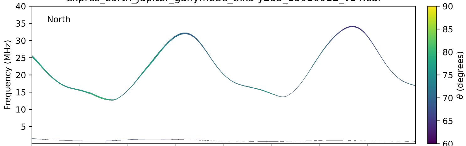
expres_earth_jupiter_ganymede_txka-y235_19920922_v14.cdf
