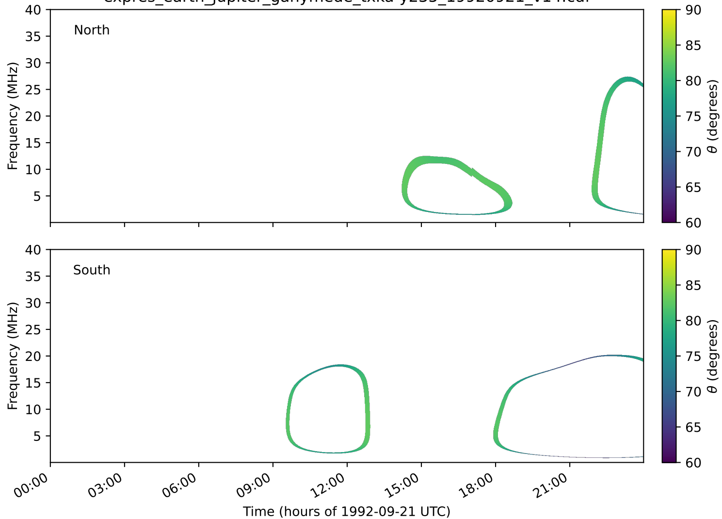
expres_earth_jupiter_ganymede_txka-y235_19920921_v14.cdf
