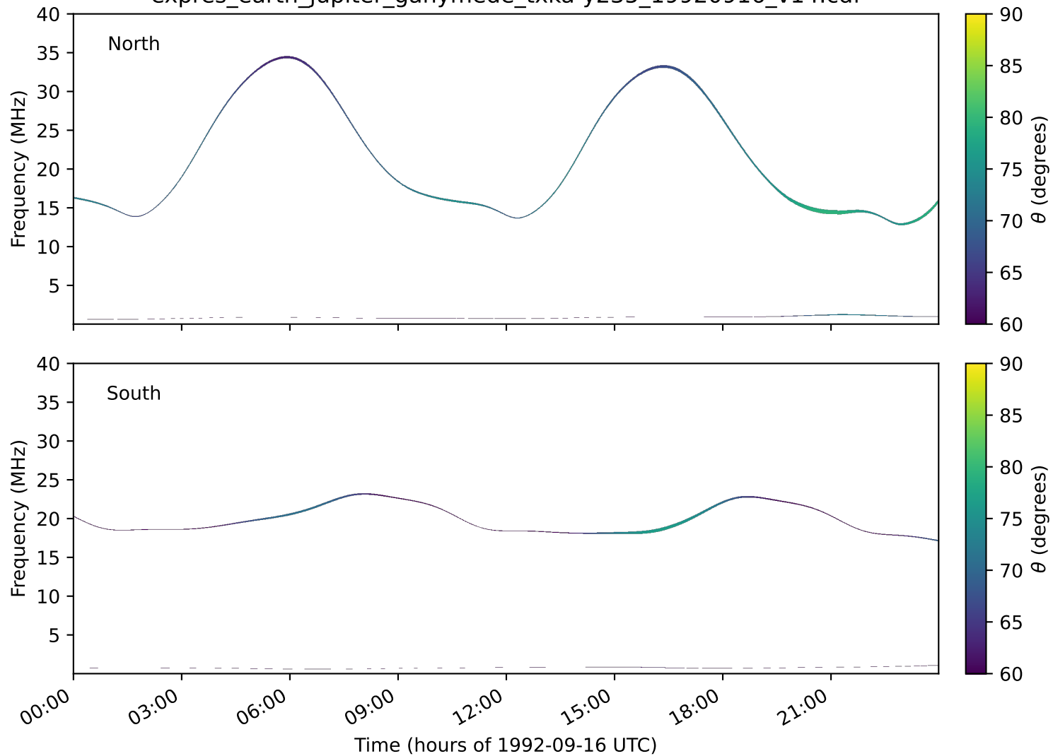
expres_earth_jupiter_ganymede_txka-y235_19920916_v14.cdf
