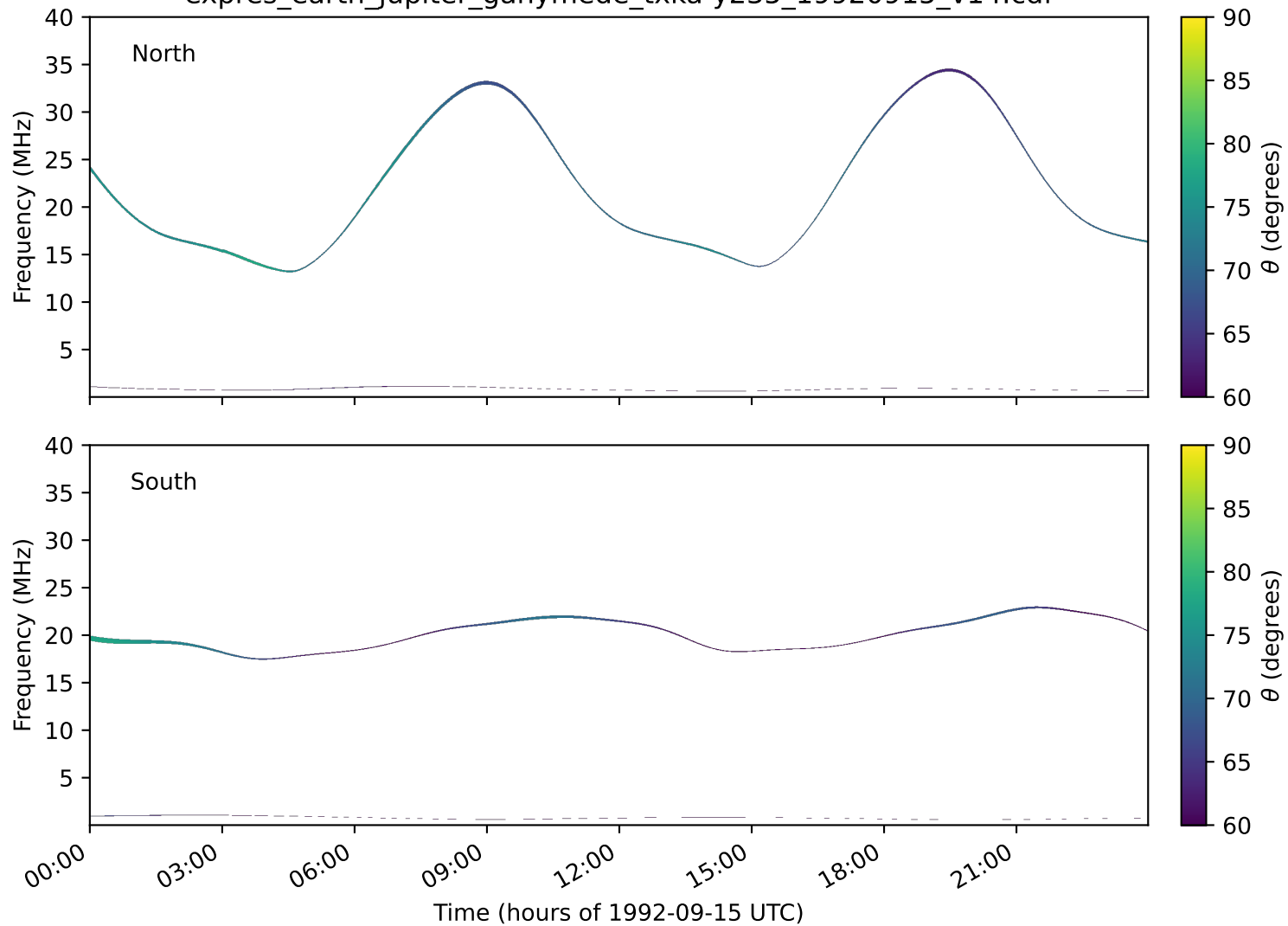
expres_earth_jupiter_ganymede_txka-y235_19920915_v14.cdf
