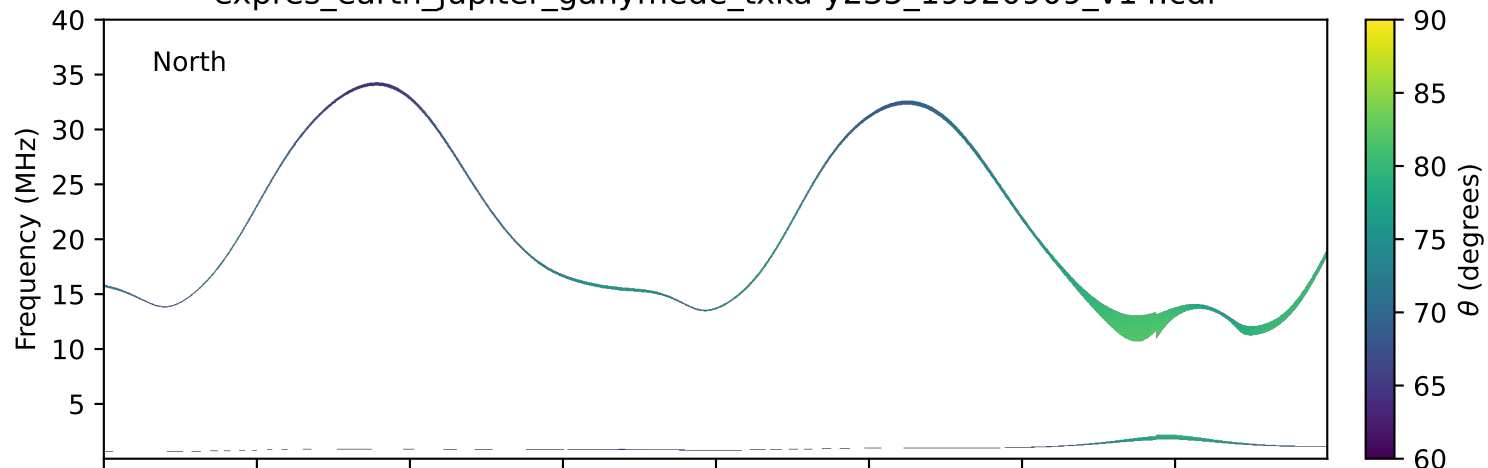
expres_earth_jupiter_ganymede_txka-y235_19920909_v14.cdf
