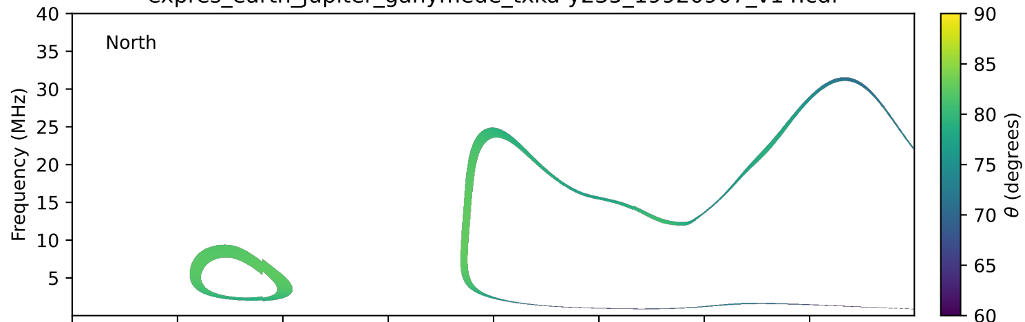
expres_earth_jupiter_ganymede_txka-y235_19920907_v14.cdf
