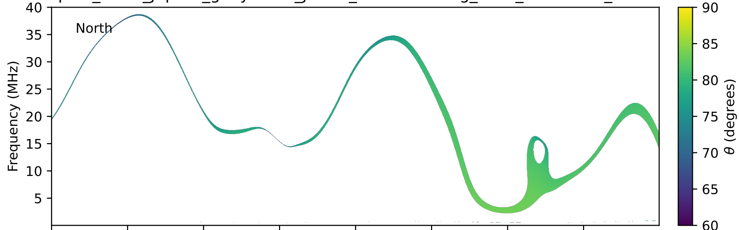
expres_earth_jupiter_ganymede_jrm33_lossc-wid1deg_3kev_19920924_v11.cdf
