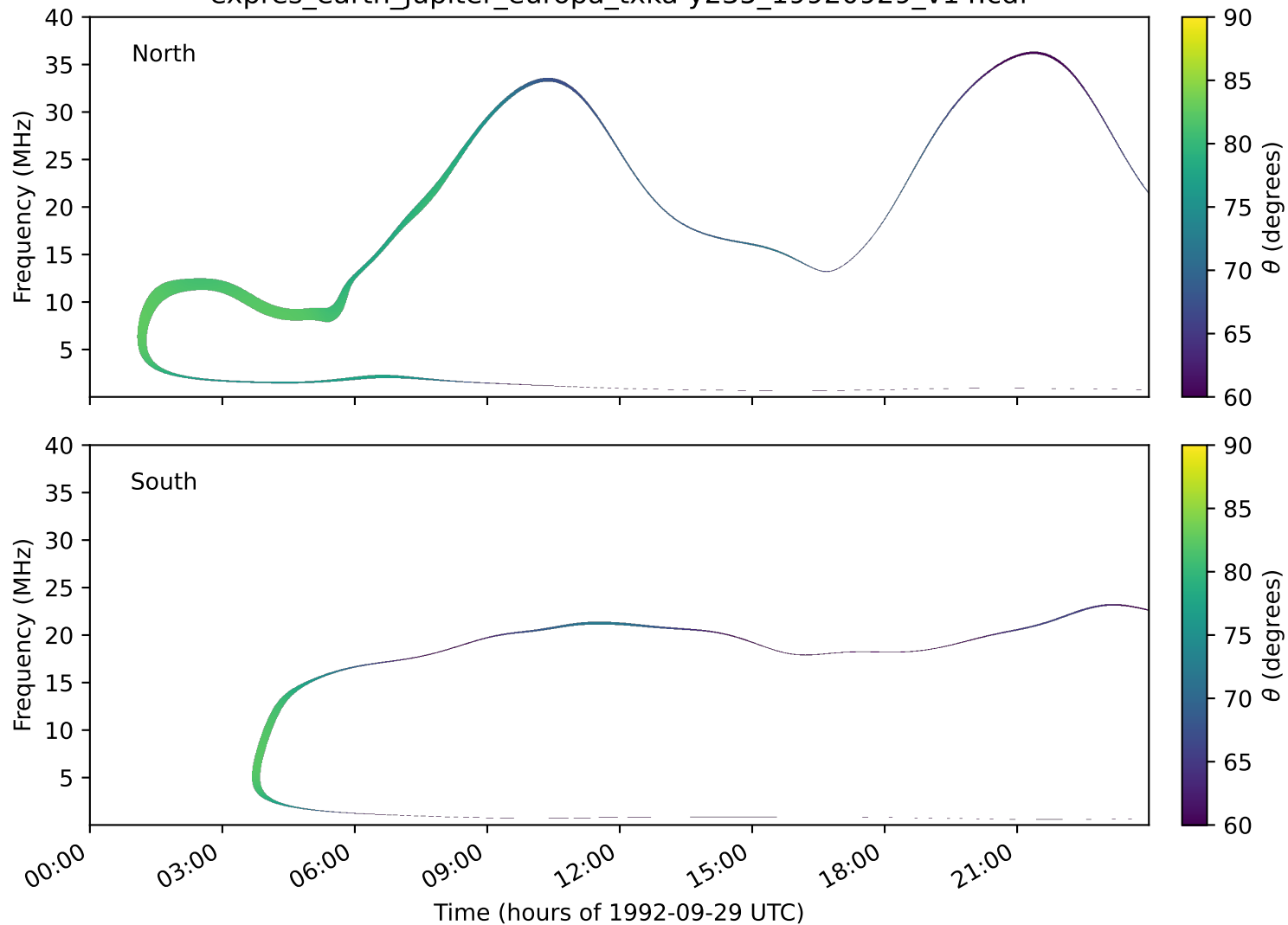
expres_earth_jupiter_europa_txka-y235_19920929_v14.cdf
