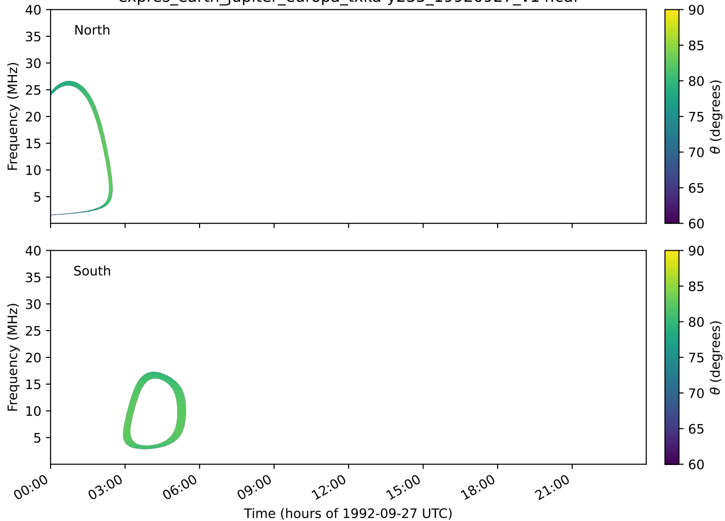
expres_earth_jupiter_europa_txka-y235_19920927_v14.cdf
