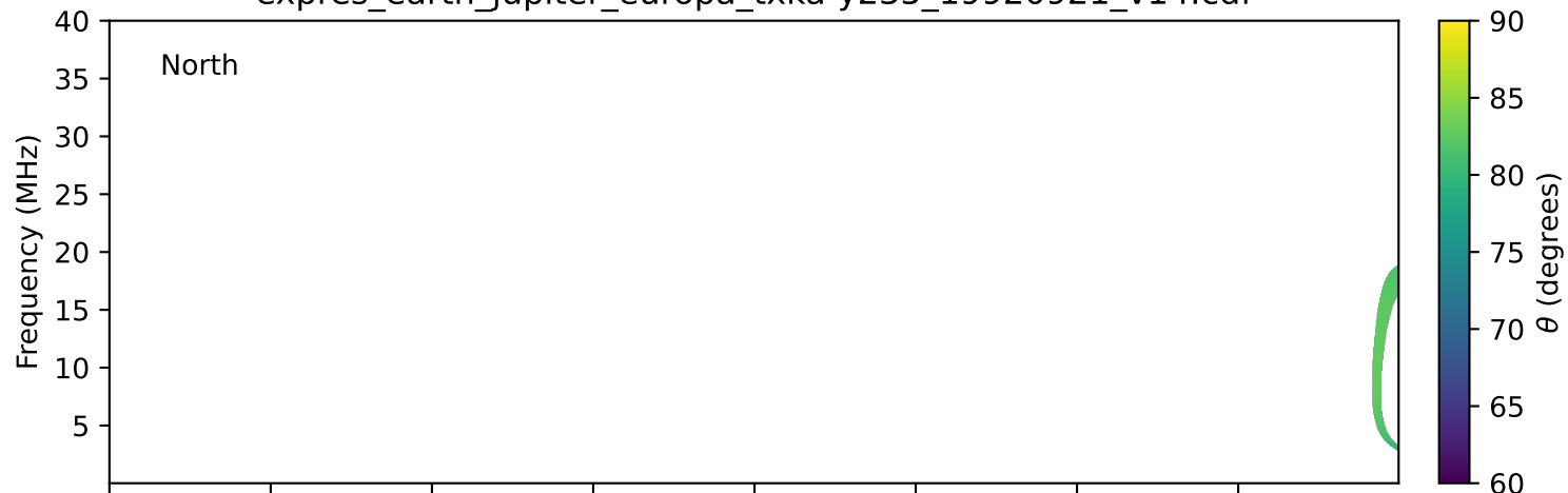
expres_earth_jupiter_europa_txka-y235_19920921_v14.cdf
