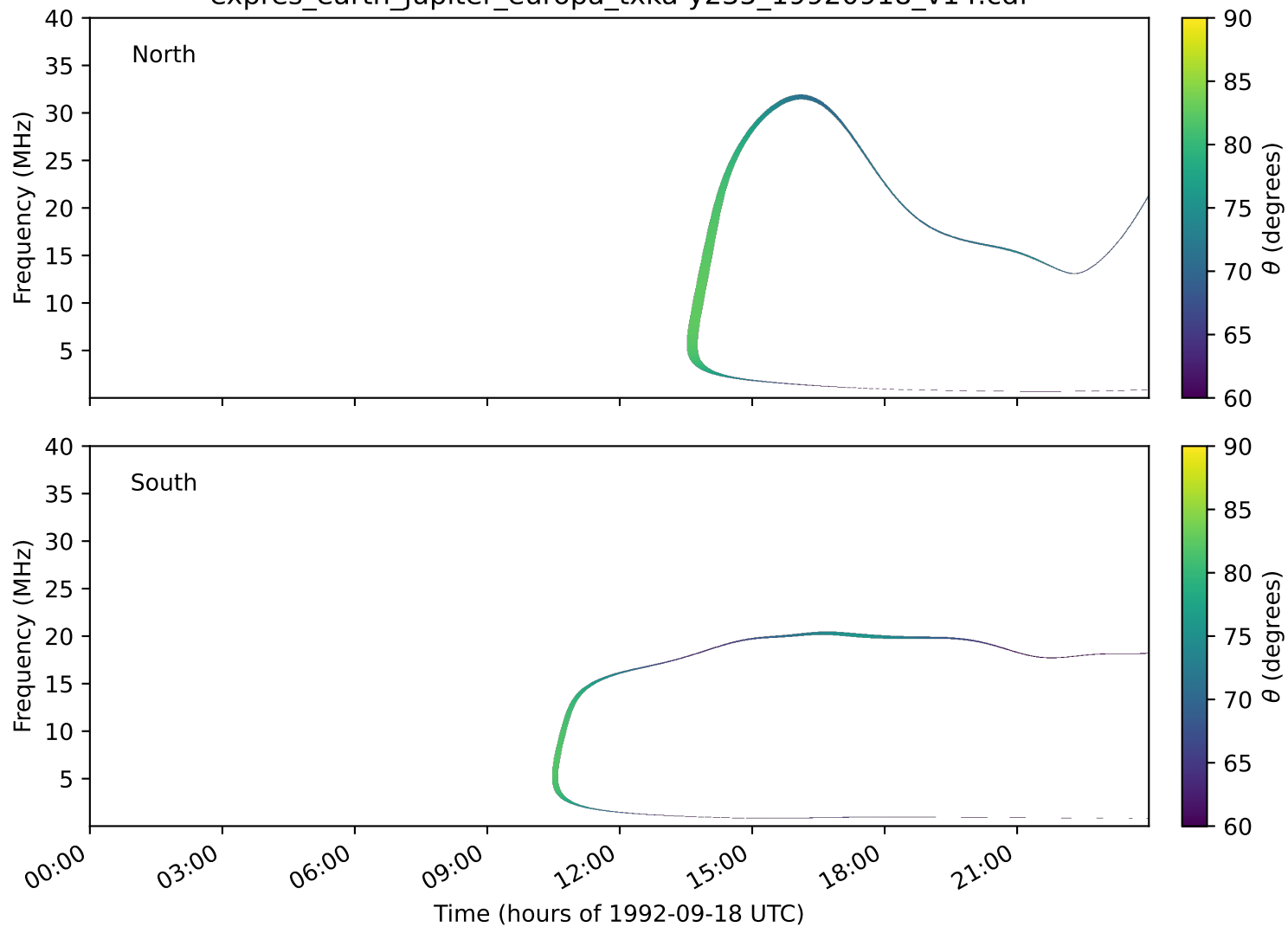
expres_earth_jupiter_europa_txka-y235_19920918_v14.cdf
