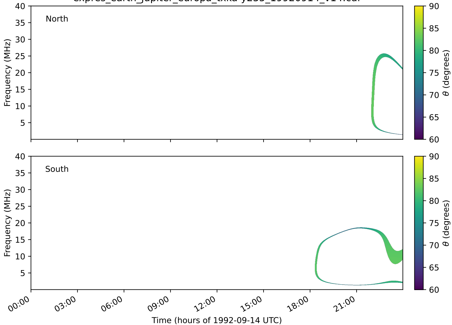
expres_earth_jupiter_europa_txka-y235_19920914_v14.cdf
