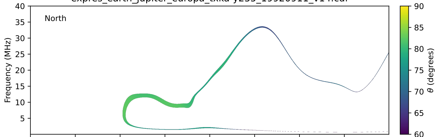
expres_earth_jupiter_europa_txka-y235_19920911_v14.cdf
