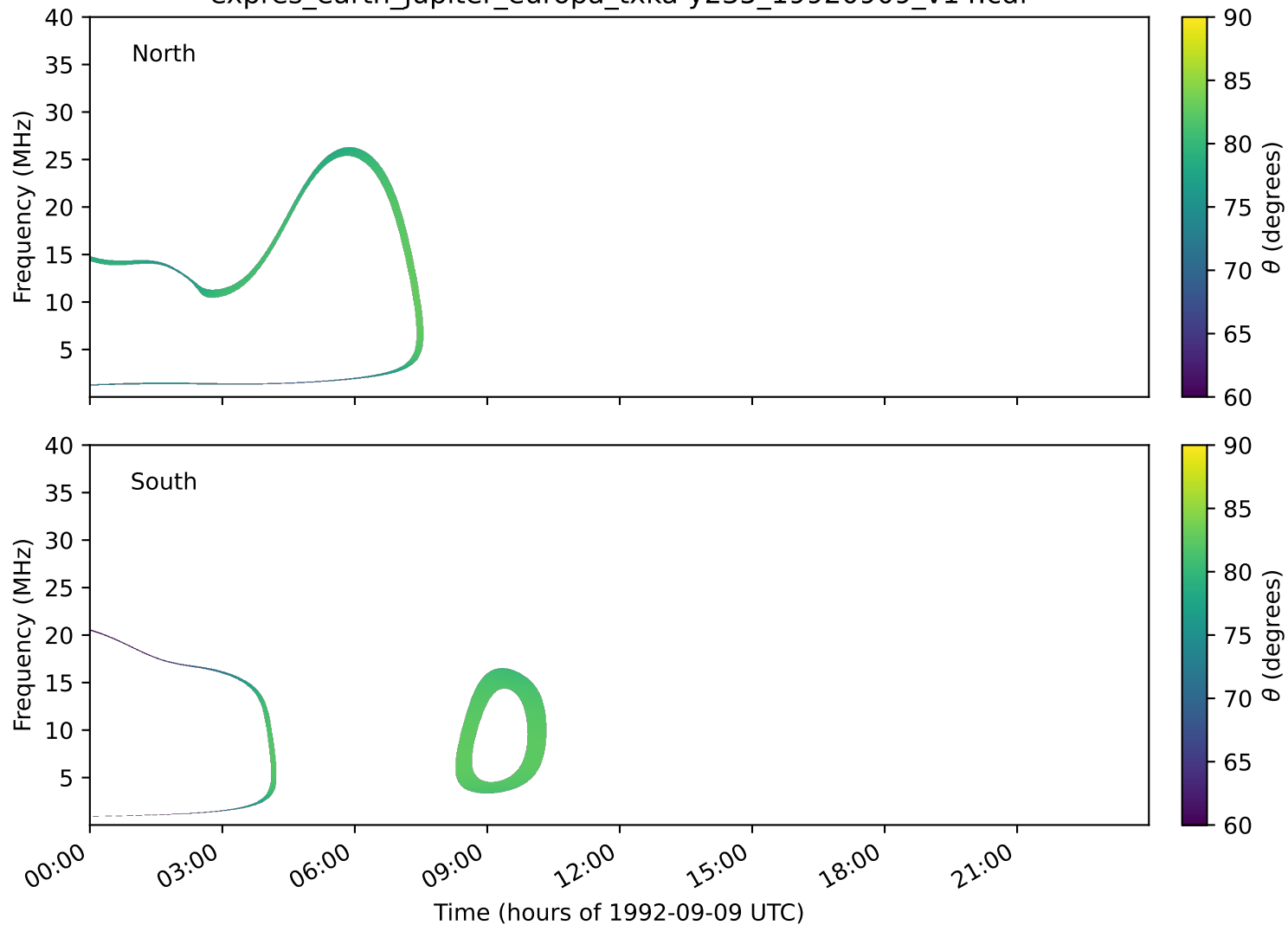
expres_earth_jupiter_europa_txka-y235_19920909_v14.cdf
