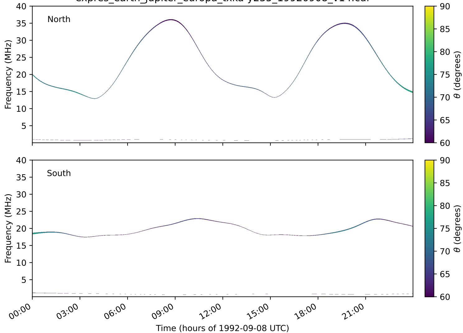
expres_earth_jupiter_europa_txka-y235_19920908_v14.cdf
