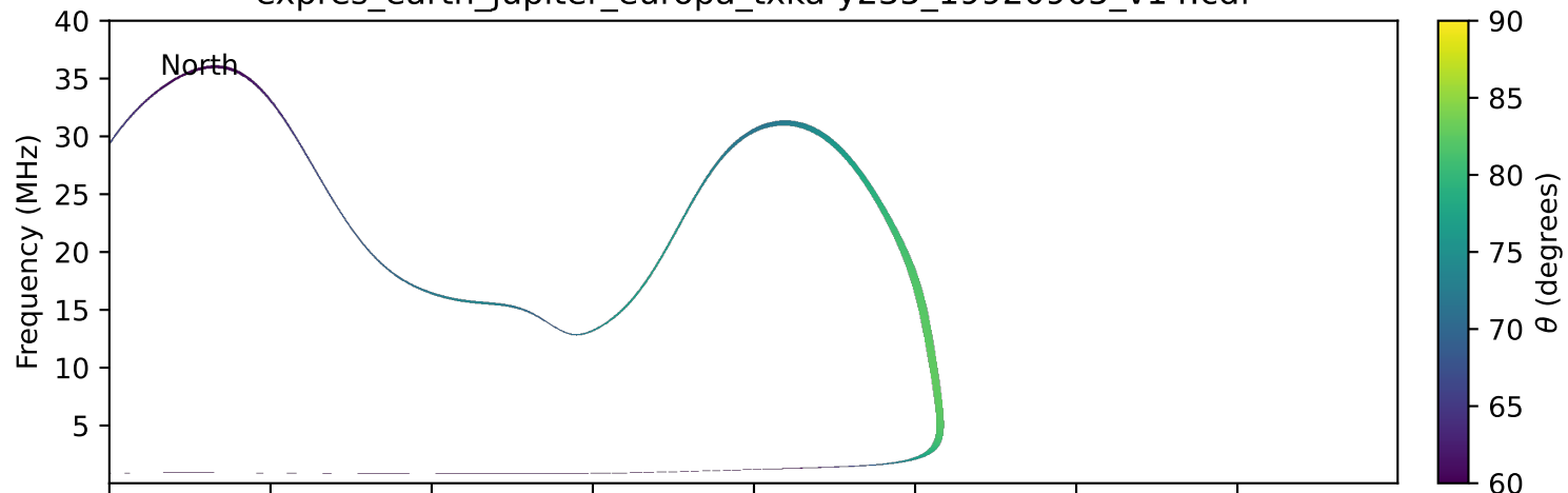
expres_earth_jupiter_europa_txka-y235_19920905_v14.cdf
