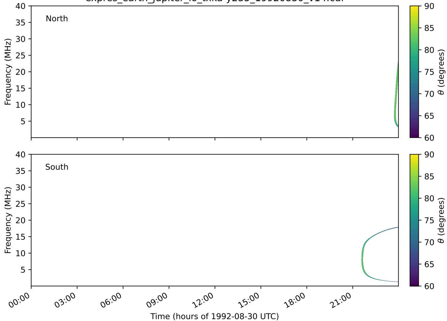
expres_earth_jupiter_io_txka-y235_19920830_v14.cdf
