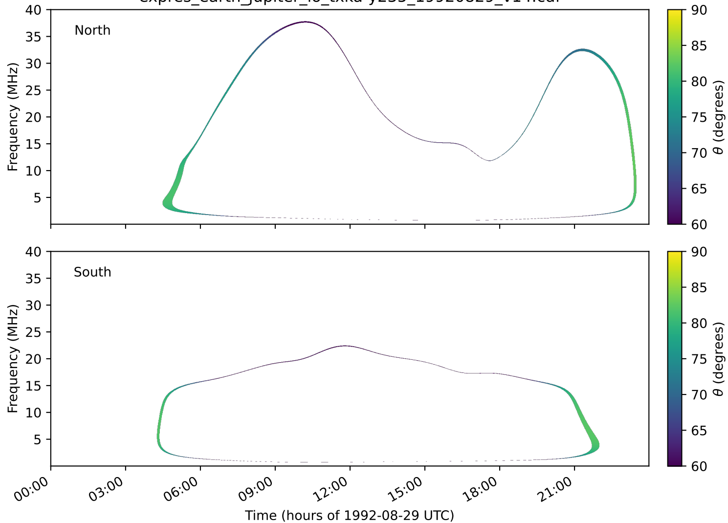
expres_earth_jupiter_io_txka-y235_19920829_v14.cdf
