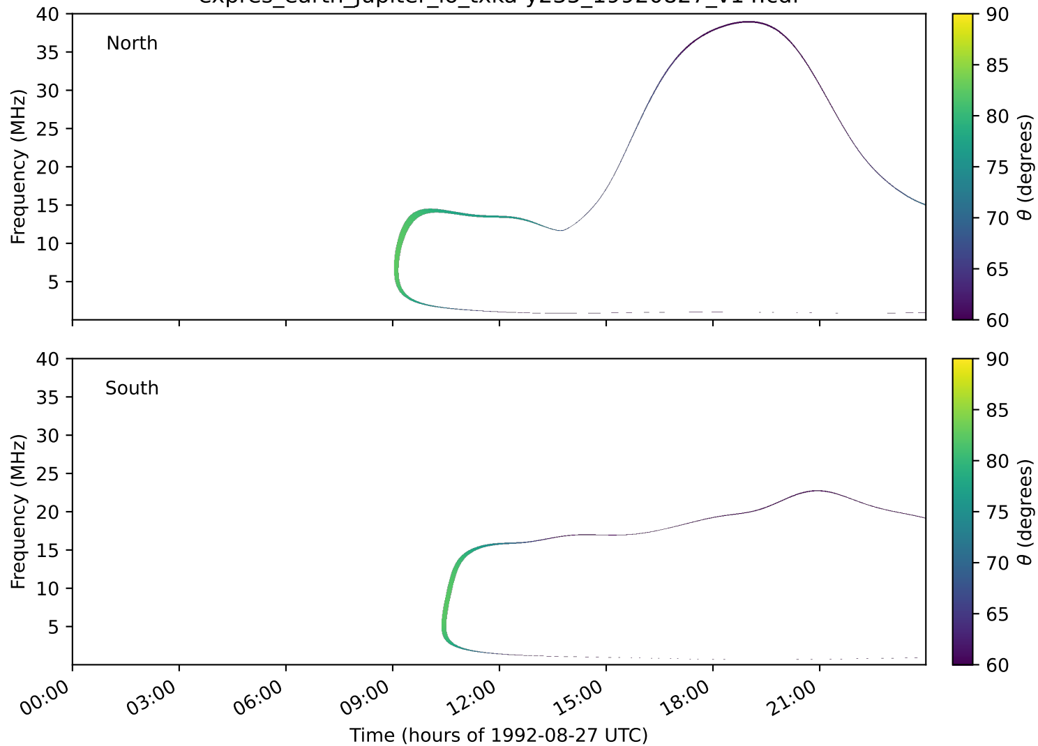
expres_earth_jupiter_io_txka-y235_19920827_v14.cdf
