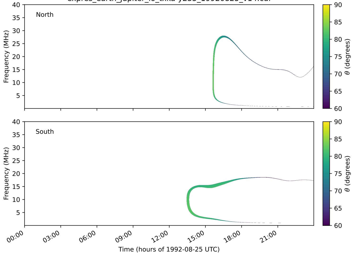
expres_earth_jupiter_io_txka-y235_19920825_v14.cdf
