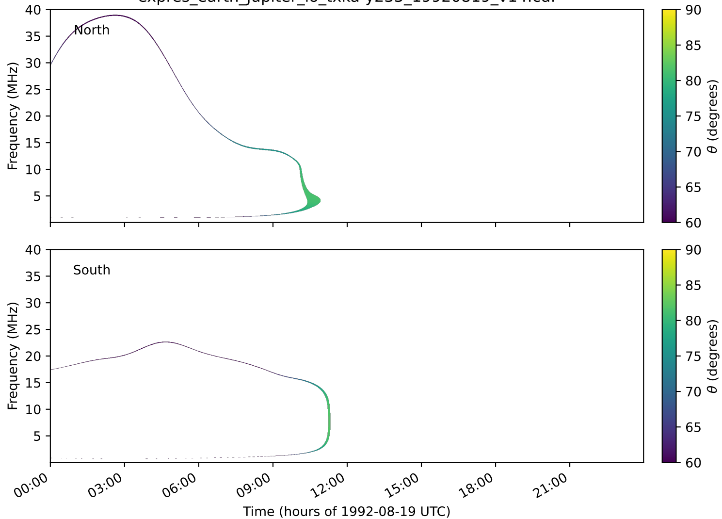
expres_earth_jupiter_io_txka-y235_19920819_v14.cdf
