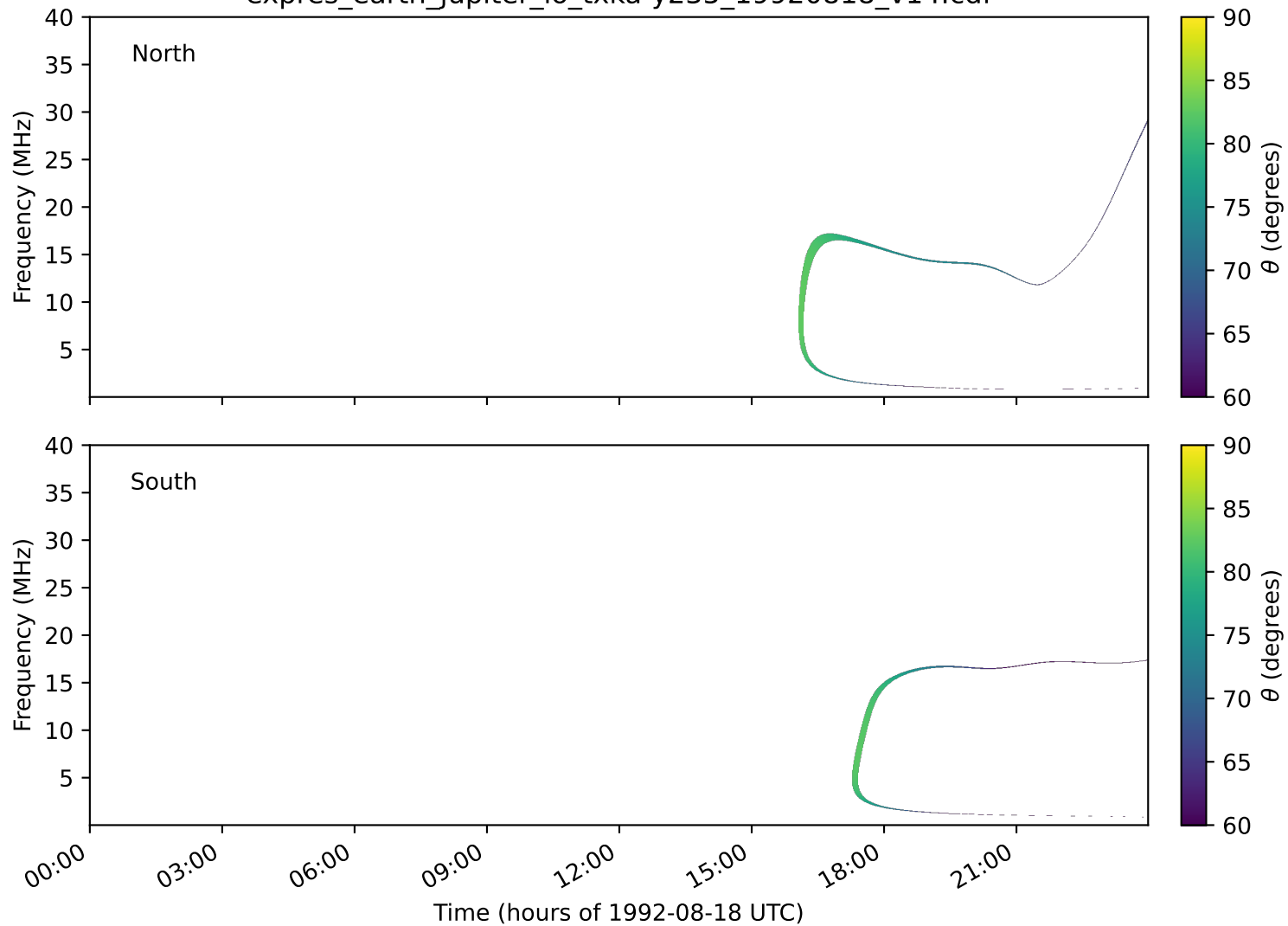
expres_earth_jupiter_io_txka-y235_19920818_v14.cdf
