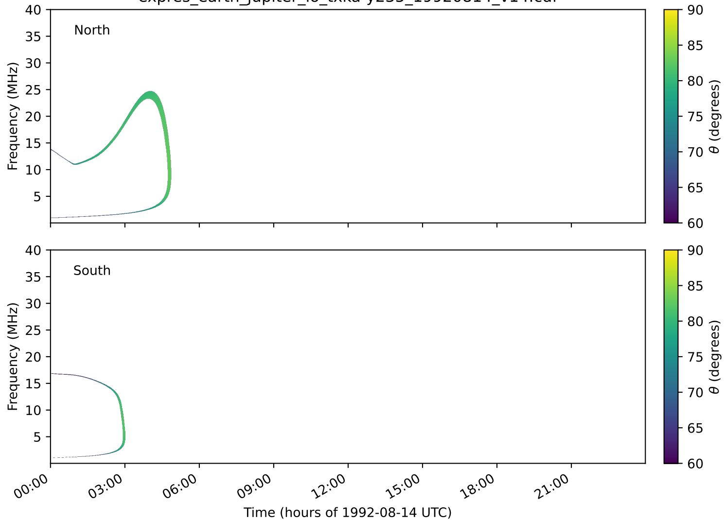
expres_earth_jupiter_io_txka-y235_19920814_v14.cdf
