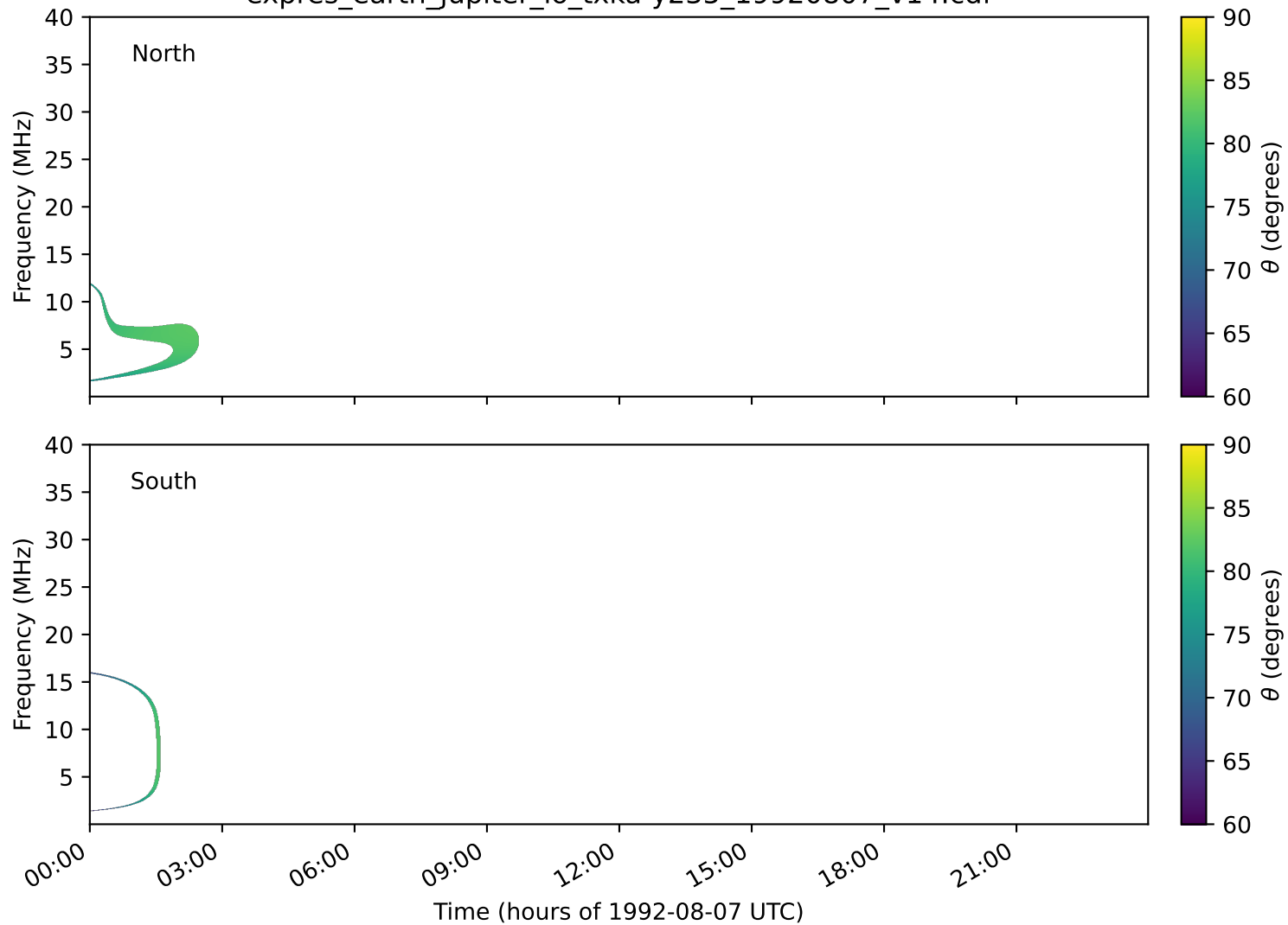
expres_earth_jupiter_io_txka-y235_19920807_v14.cdf
