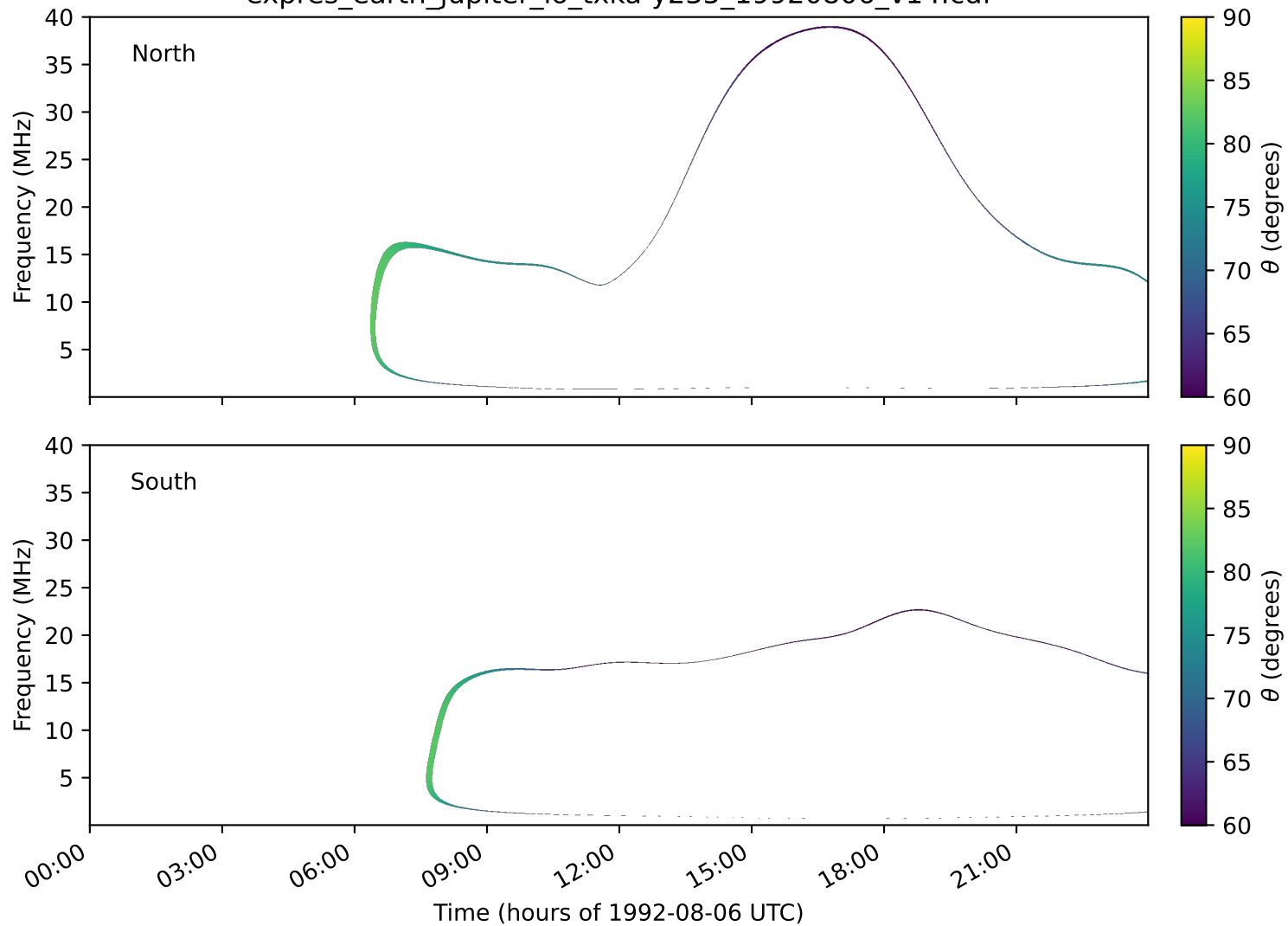
expres_earth_jupiter_io_txka-y235_19920806_v14.cdf
