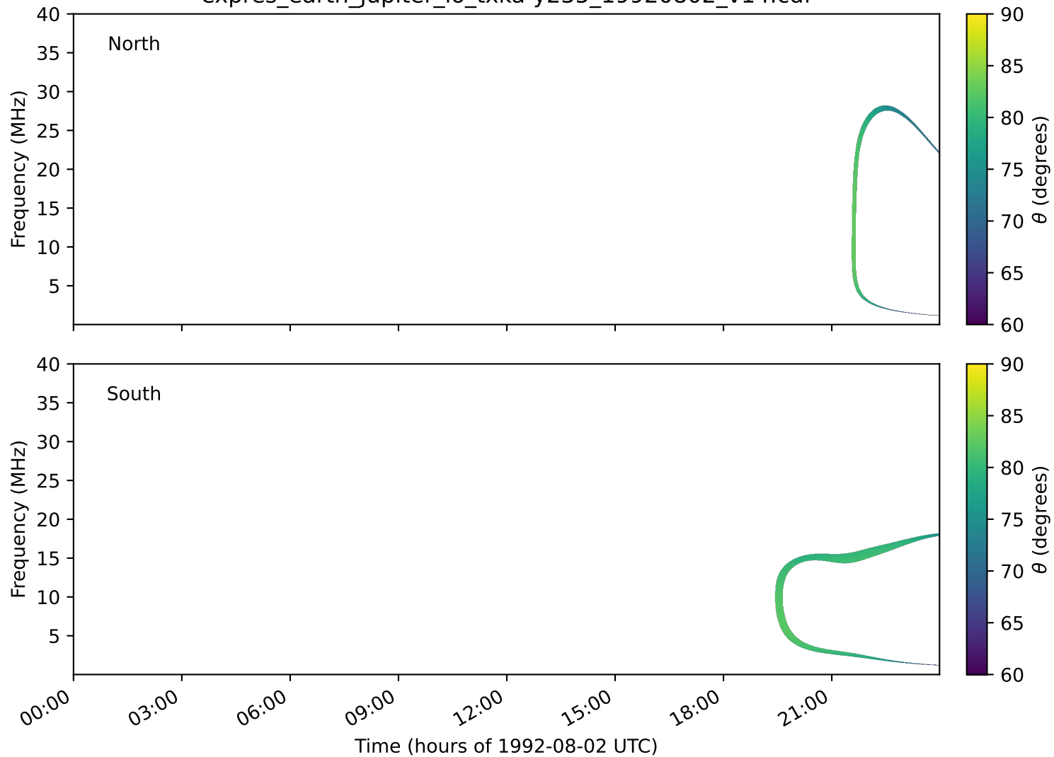
expres_earth_jupiter_io_txka-y235_19920802_v14.cdf
