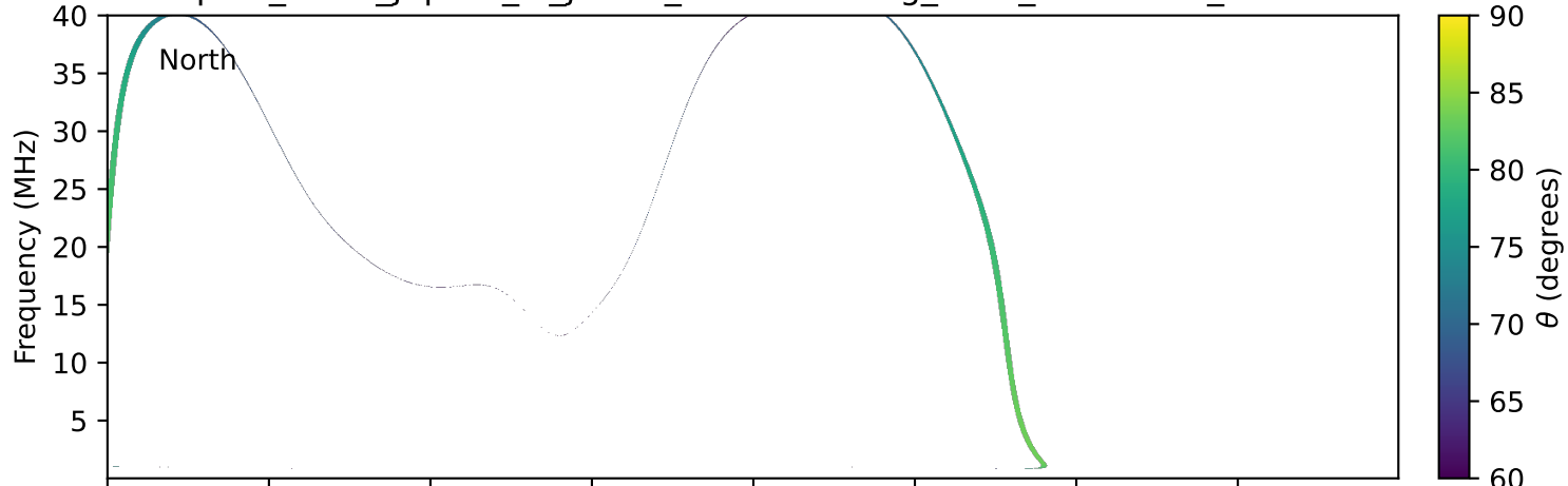
expres_earth_jupiter_io_jrm33_lossc-wid1deg_3kev_19920831_v11.cdf
