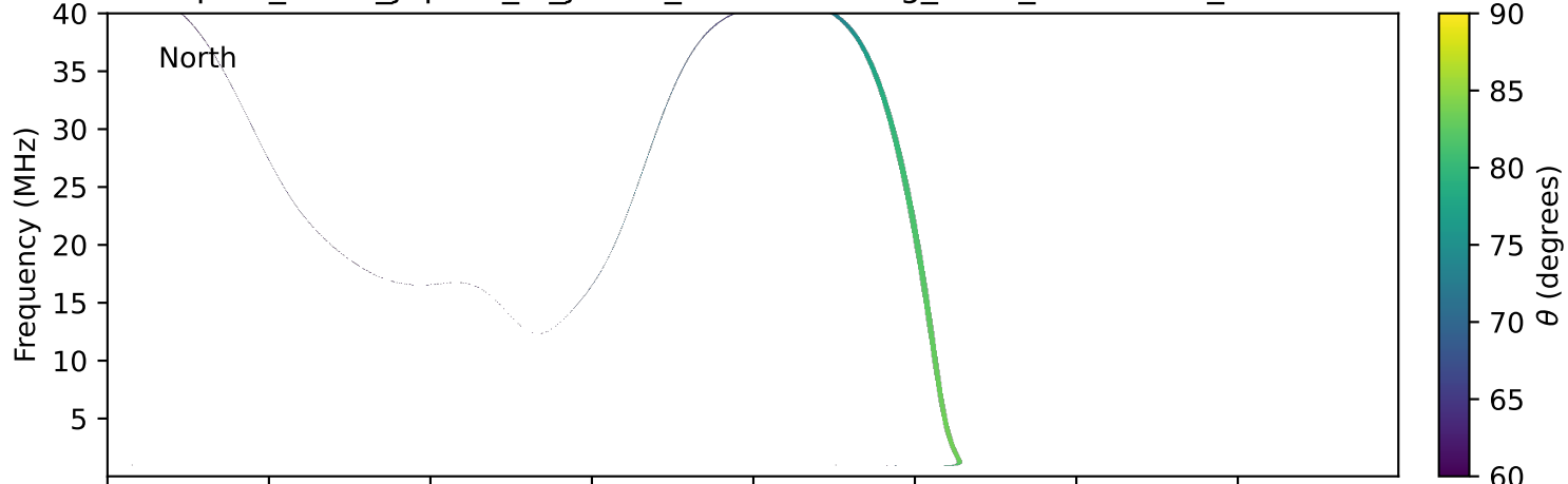
expres_earth_jupiter_io_jrm33_lossc-wid1deg_3kev_19920824_v11.cdf
