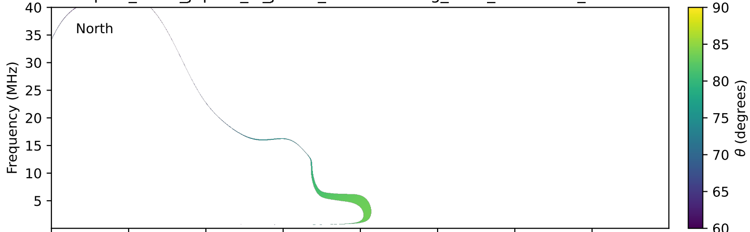
expres_earth_jupiter_io_jrm33_lossc-wid1deg_3kev_19920819_v11.cdf
