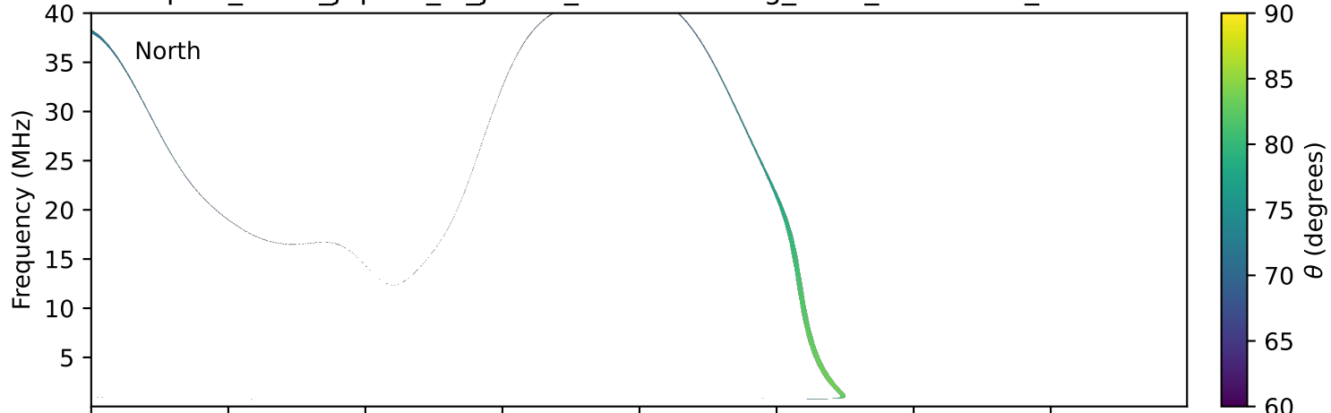
expres_earth_jupiter_io_jrm33_lossc-wid1deg_3kev_19920817_v11.cdf
