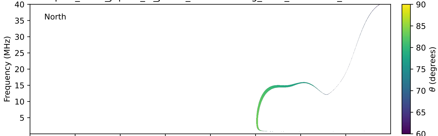
expres_earth_jupiter_io_jrm33_lossc-wid1deg_3kev_19920804_v11.cdf
