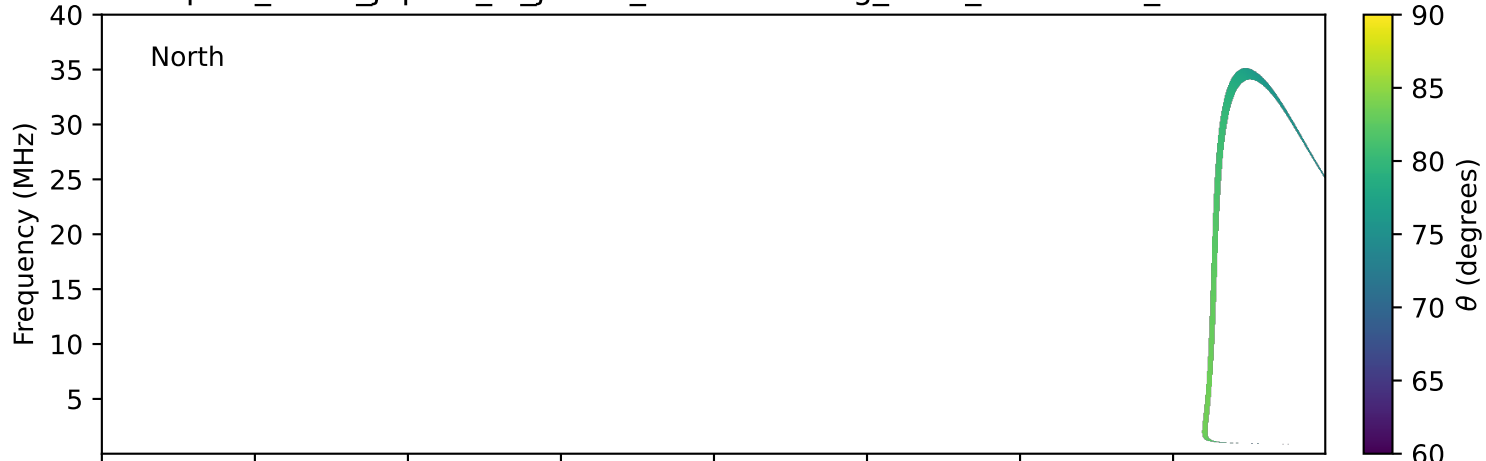
expres_earth_jupiter_io_jrm33_lossc-wid1deg_3kev_19920802_v11.cdf
