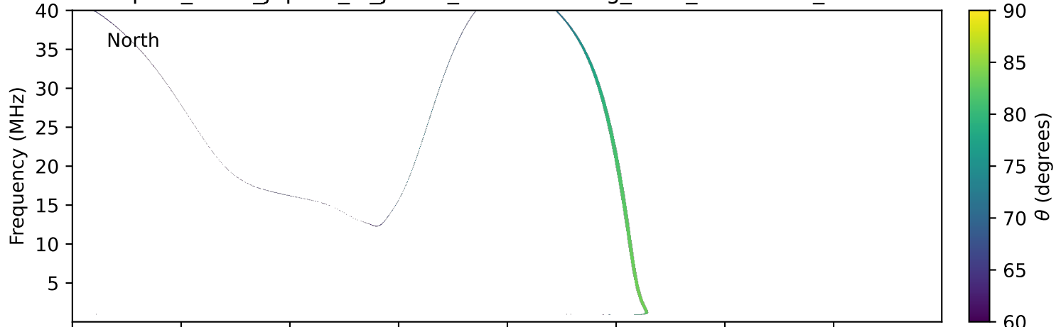
expres_earth_jupiter_io_jrm09_lossc-wid1deg_3kev_19920824_v11.cdf
