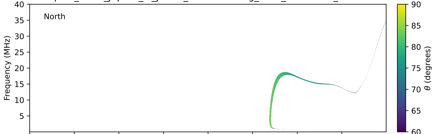
expres_earth_jupiter_io_jrm09_lossc-wid1deg_3kev_19920818_v11.cdf
