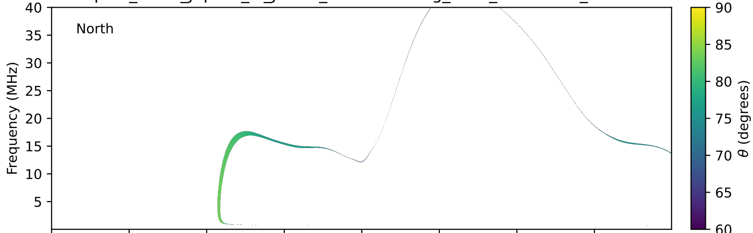
expres_earth_jupiter_io_jrm09_lossc-wid1deg_3kev_19920806_v11.cdf
