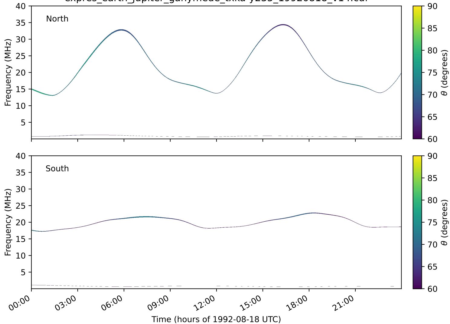
expres_earth_jupiter_ganymede_txka-y235_19920818_v14.cdf
