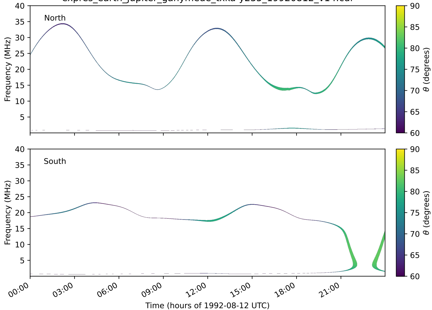
expres_earth_jupiter_ganymede_txka-y235_19920812_v14.cdf
