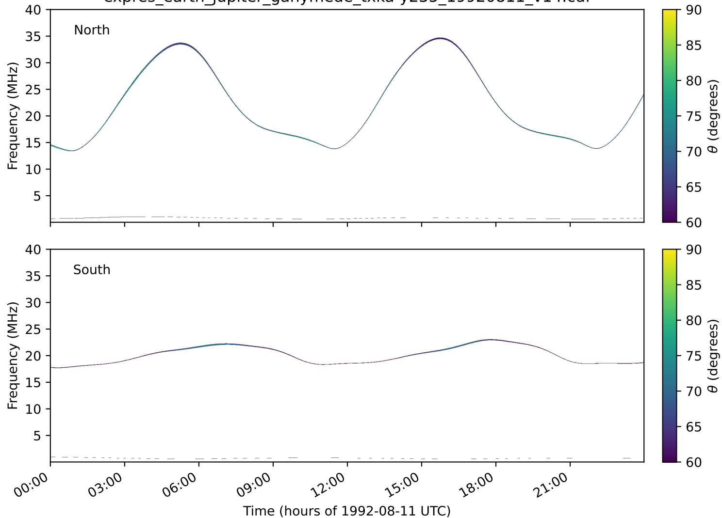
expres_earth_jupiter_ganymede_txka-y235_19920811_v14.cdf
