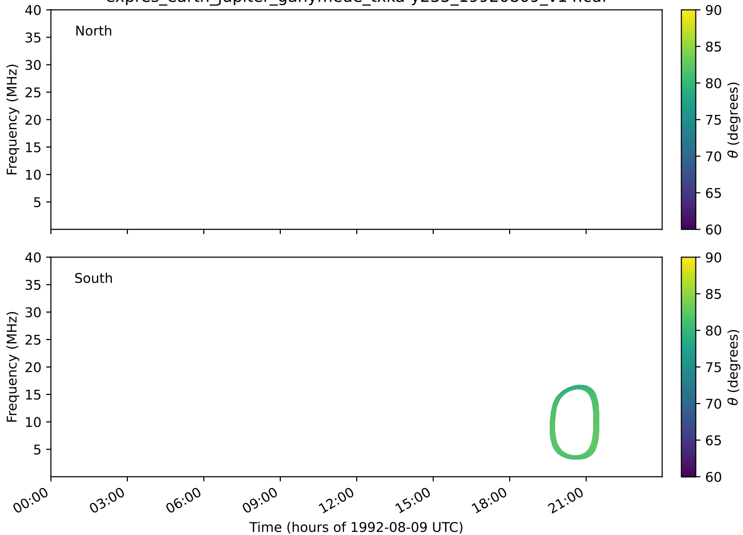
expres_earth_jupiter_ganymede_txka-y235_19920809_v14.cdf
