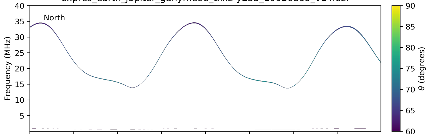
expres_earth_jupiter_ganymede_txka-y235_19920805_v14.cdf
