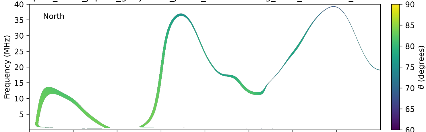
expres_earth_jupiter_ganymede_jrm33_lossc-wid1deg_3kev_19920824_v11.cdf
