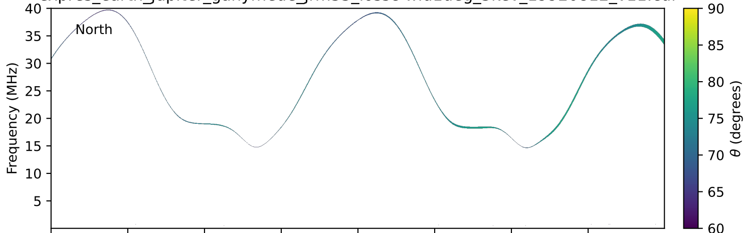
expres_earth_jupiter_ganymede_jrm33_lossc-wid1deg_3kev_19920812_v11.cdf
