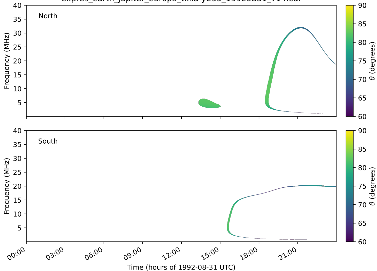
expres_earth_jupiter_europa_txka-y235_19920831_v14.cdf
